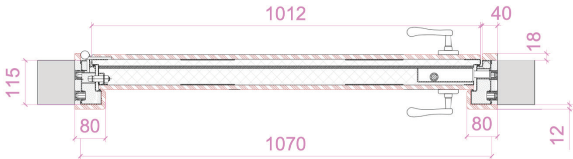
Cross section
