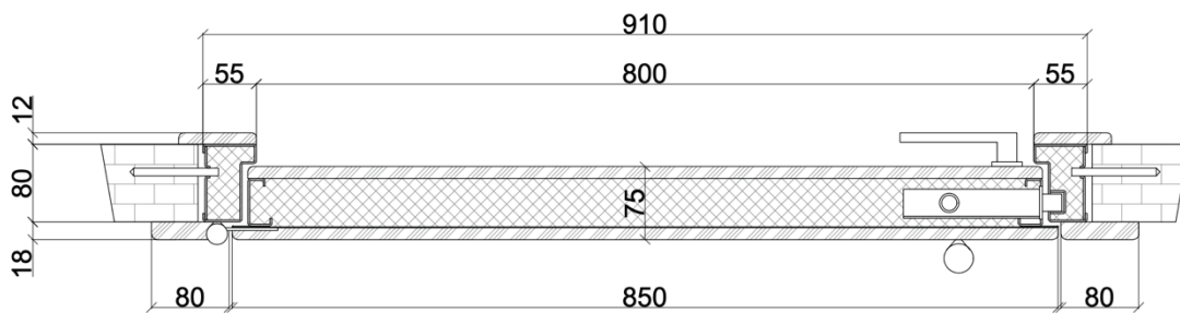
Cross section
